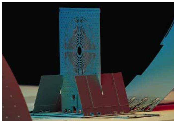
MICROSCOPICAL LENS is 280 microns in diameter and sits atop a silicon microchip.
